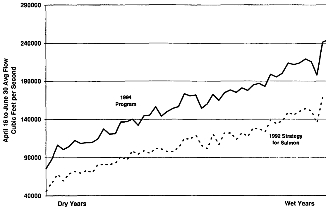
Figure 5-1 Equivalent Spring Flows at Lower Granite Dam
