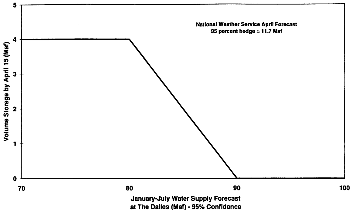
Figure 5-2 Storage Volume Required for Columbia River Flow Augmentation
