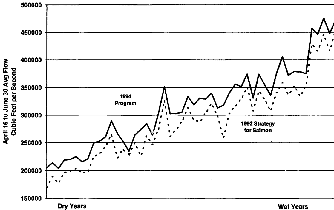
Figure 5-3 Equivalent Spring Flows at The Dalles Dam
