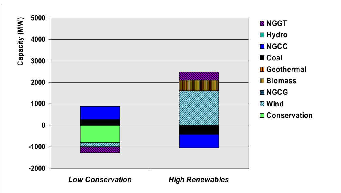
Figure 7: Incremental 2005-24 capacity compared to the base case
