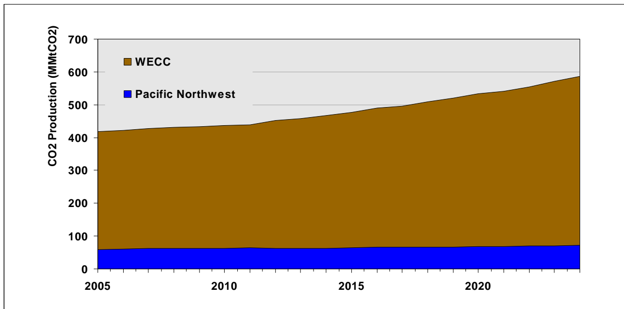
Figure 5: Forecast WECC and Northwest power system CO 2 production
