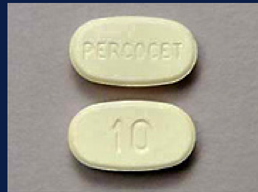
oxycodone
